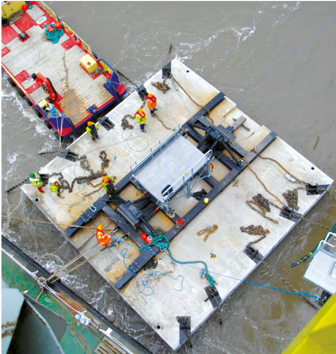
River Mersey, 2014, 12m x 12m bridge landing pontoon installation.
