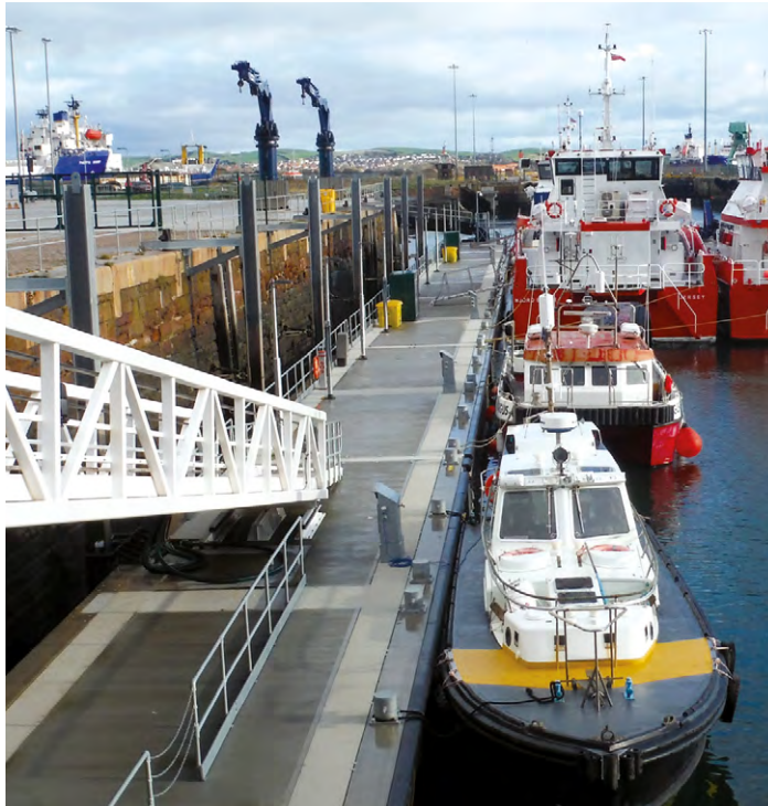
Barrow, 2017, 5.5m wide DockMaster concrete pontoons.
